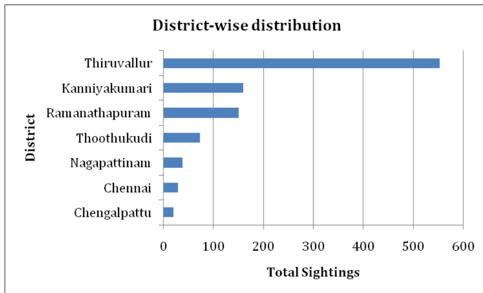
Figure 8: District wise relative abundance of Ruddy Turnstone
