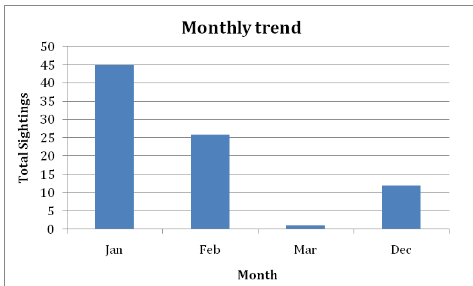
Figure 19: Monthly trend in occurrence of Common Pochard
