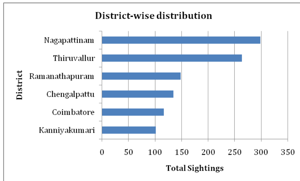
Figure 26: District wise relative abundance of Curlew Sandpiper
