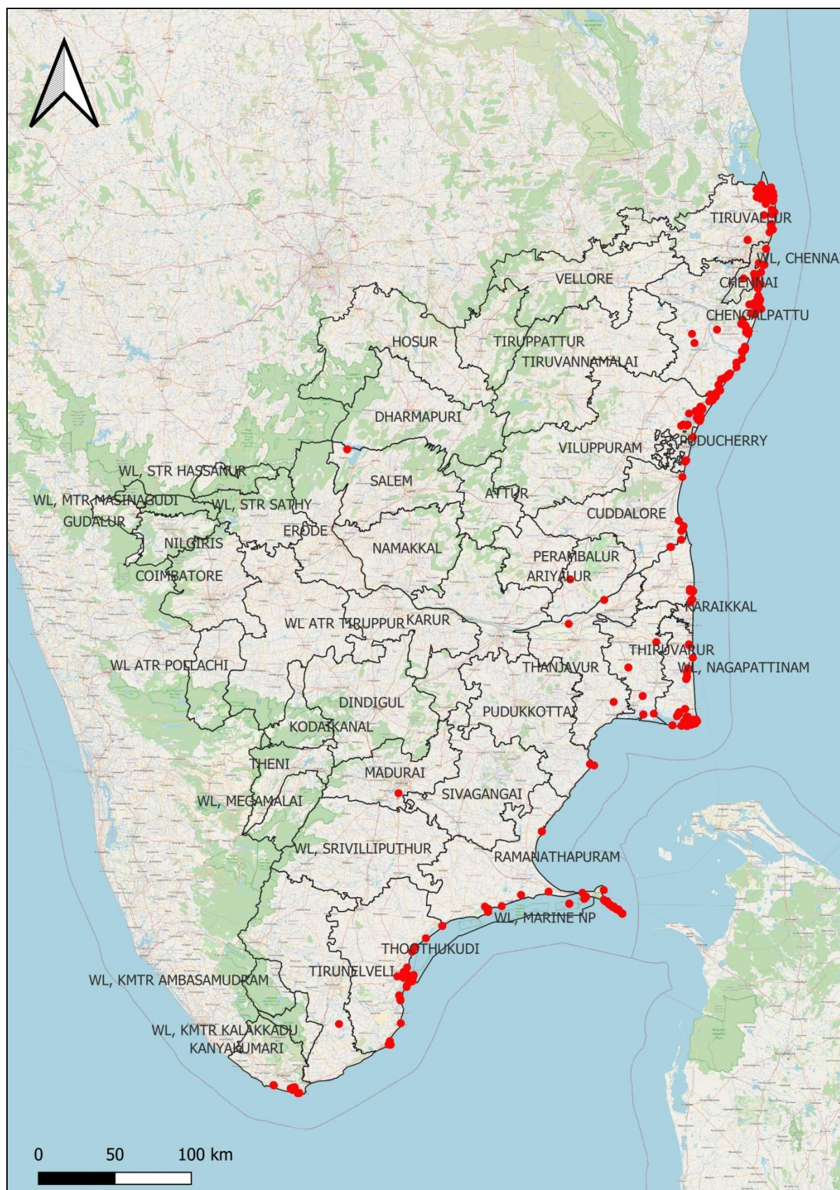
Figure 11: Geographical distribution of Eurasian Curlew (2015-2025)
