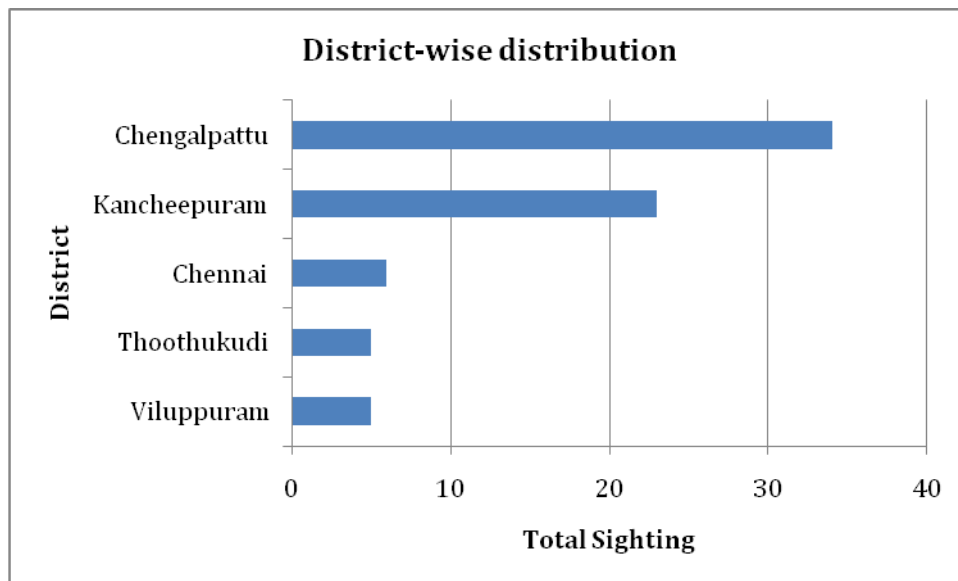
Figure 20: District wise relative abundance of Common Pochard
