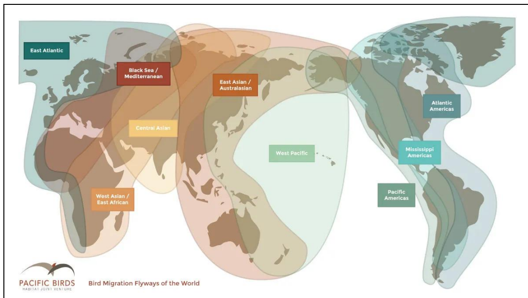
Figure1: Bird Migration Flyways of the World (Source: Pacific Birds)
