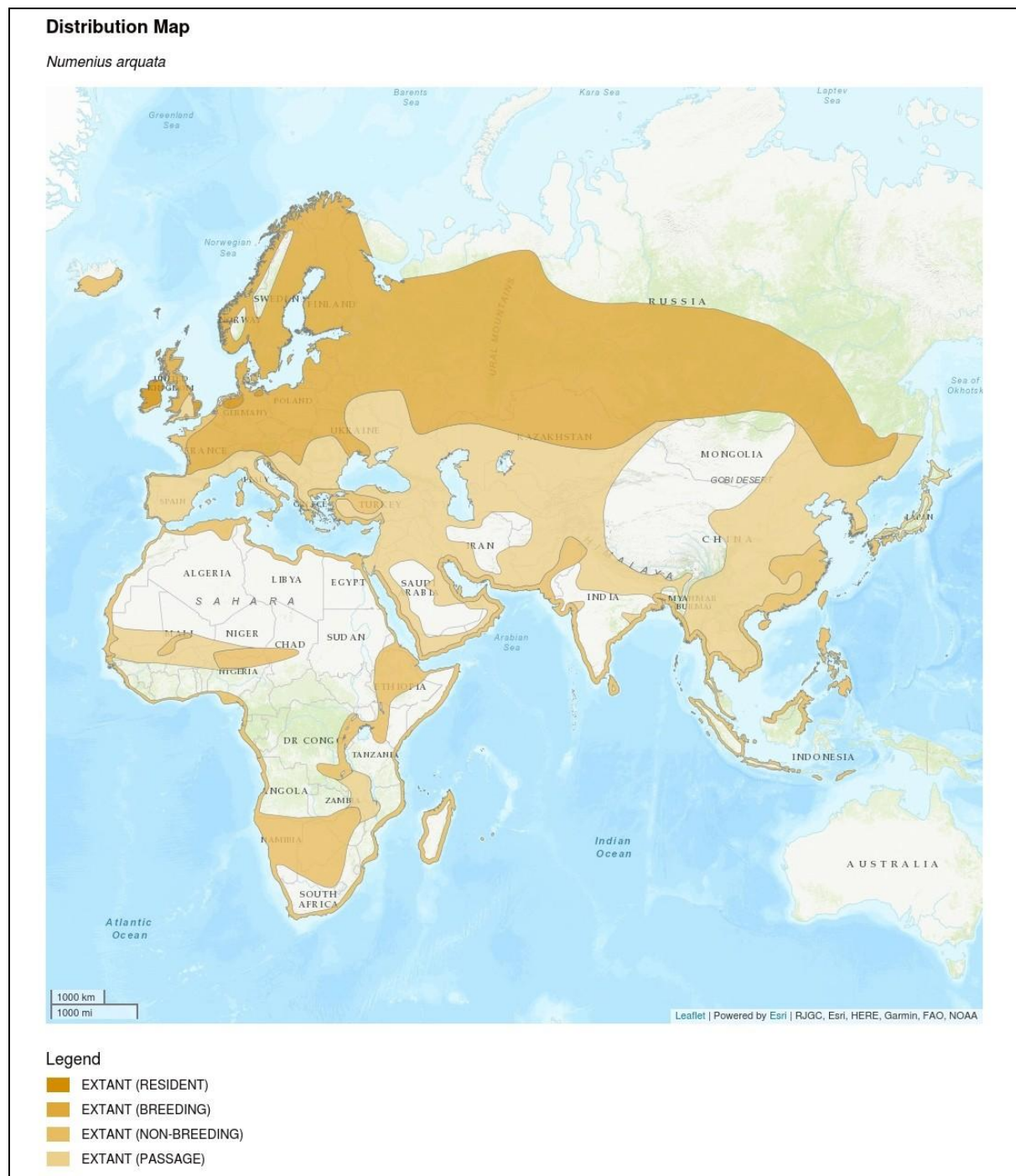
Figure 10: Distribution map adopted from IUCN (Source: BirdLife International. 2017)
