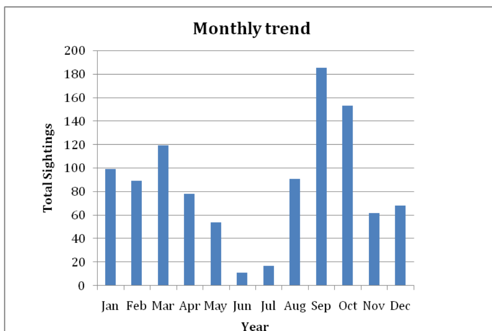
Figure 7: Monthly trend in occurrence of Ruddy Turnstone
