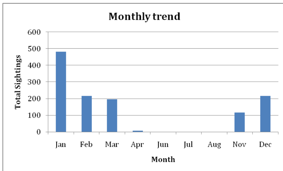
Figure 31: Monthly trend in occurrence of Bar-headed Goose
