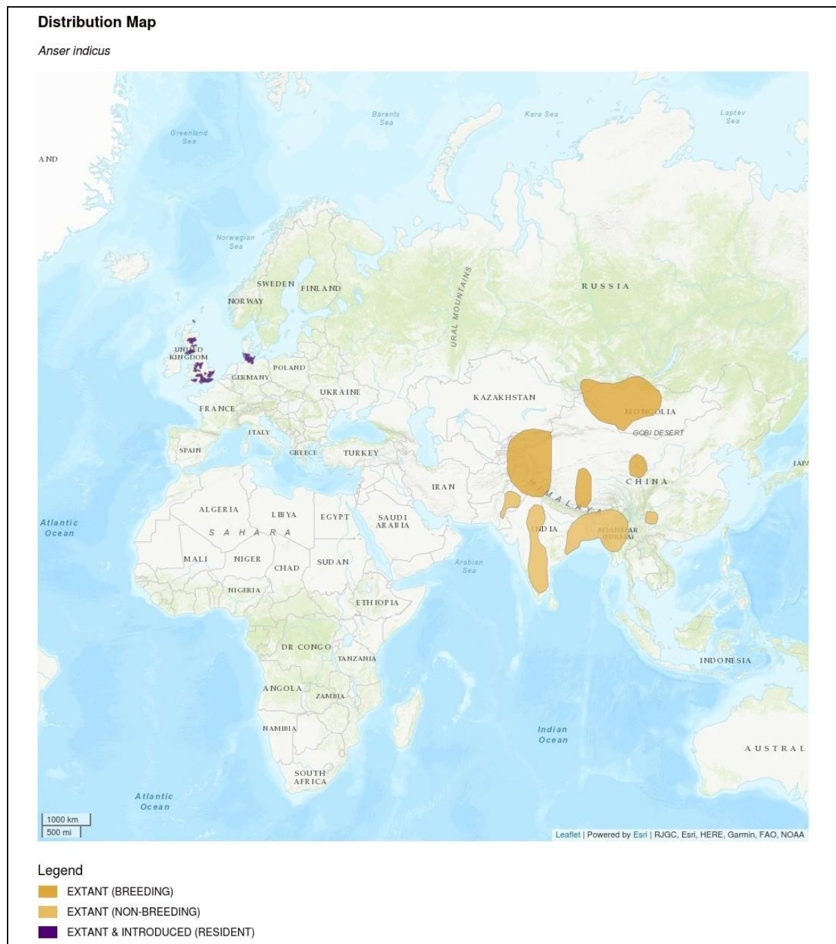
Figure 28: Distribution map adopted from IUCN, BirdLife International, 2018)
