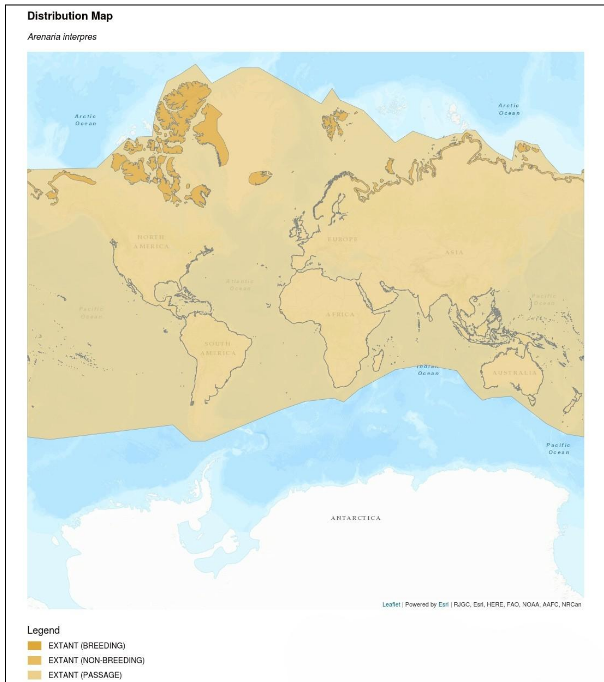
Figure 4: Distribution map adopted from IUCN, (Source: BirdLife International, 2024)
