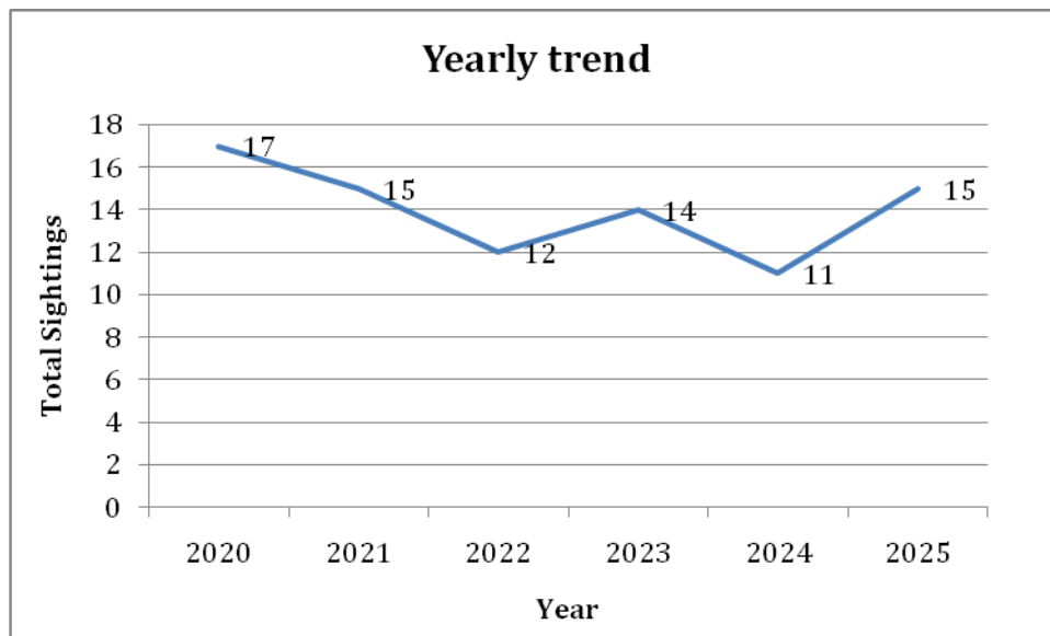
Figure 18: Yearly trend in occurrence of Common Pochard
