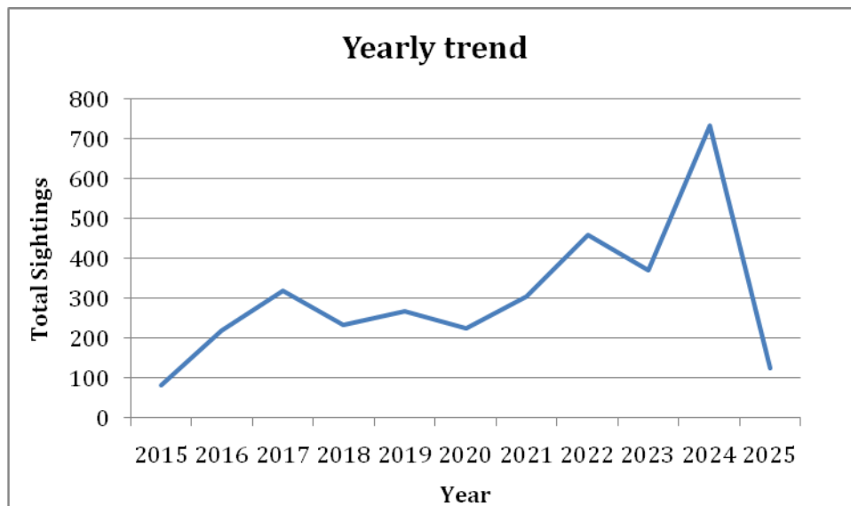
Figure 12: Yearly trend in occurrence of Eurasian Curlew
