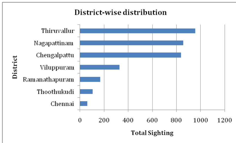
Figure 14: District wise relative abundance of Eurasian Curlew
