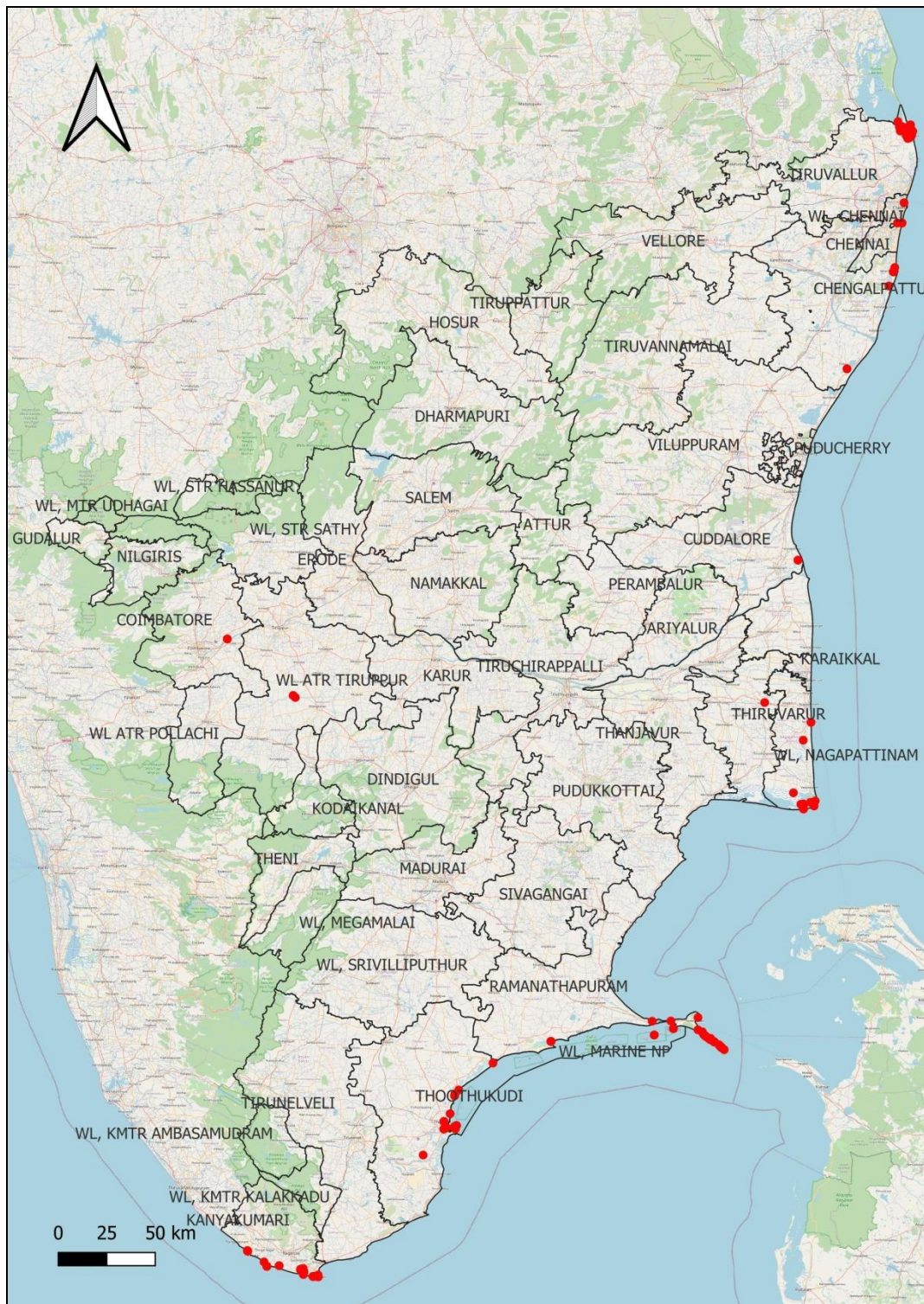
Figure 5: Geographical distribution of Ruddy Turnstone (2015-2025)
