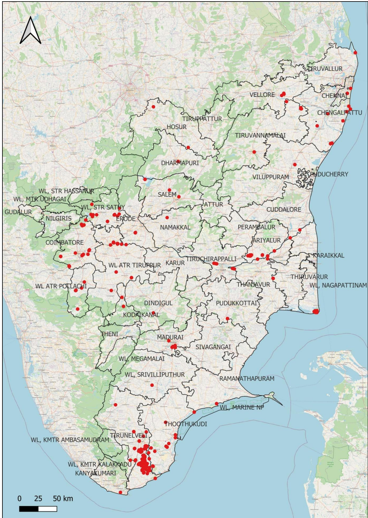
Figure 29: Geographical distribution of Bar-headed Goose (2015-2025)
