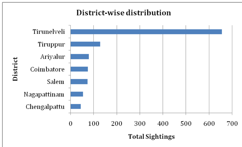
Figure 32: District wise relative abundance of Bar-headed Goose
