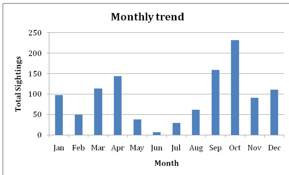
Figure 25: Monthly trend in occurrence of Curlew Sandpiper
