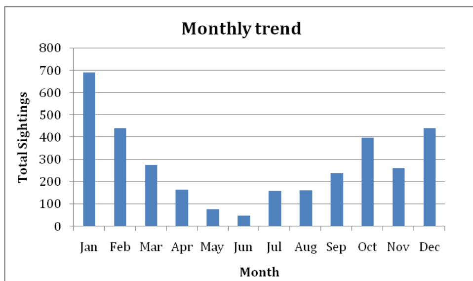
Figure 13: Monthly trend in occurrence of Eurasian Curlew
