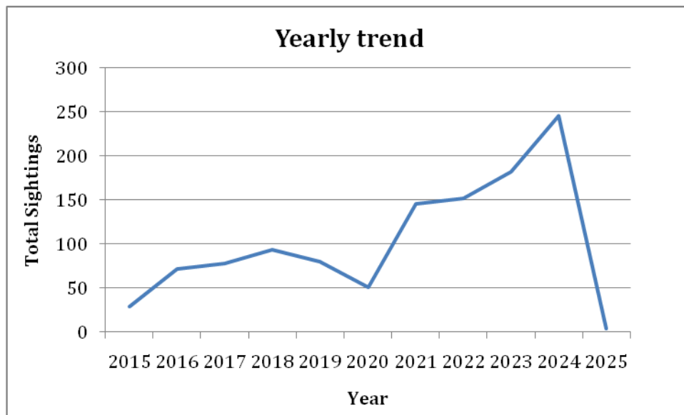
Figure 24: Yearly trend in occurrence of Curlew Sandpiper
