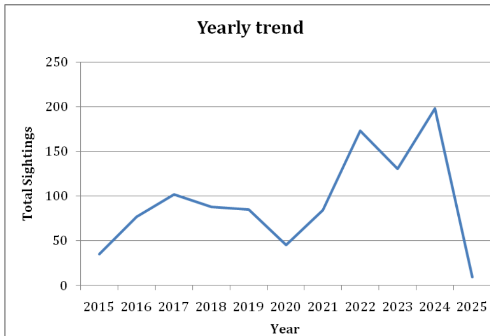
Figure 6: Yearly trend in occurrence of Ruddy Turnstone
