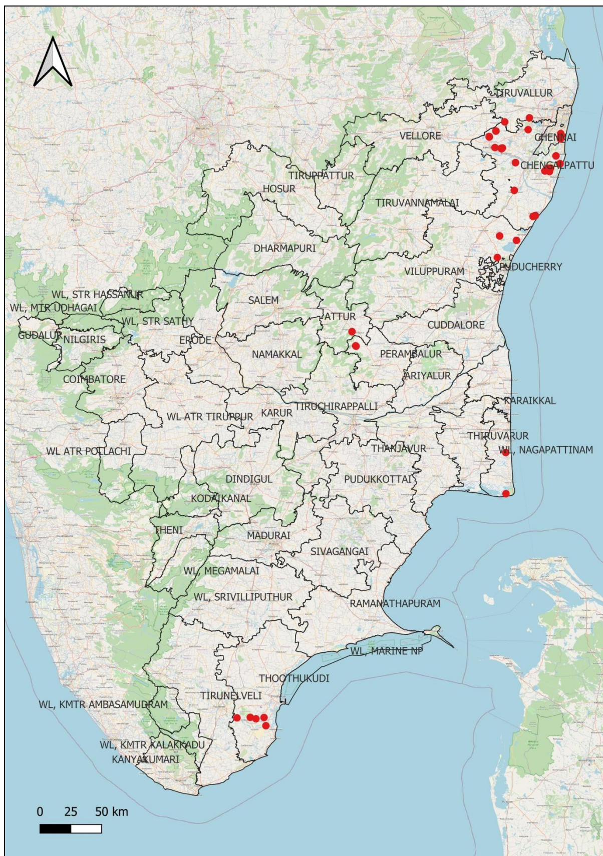
Figure 17: Geographical distribution of Common Pochard (2015-2025)
