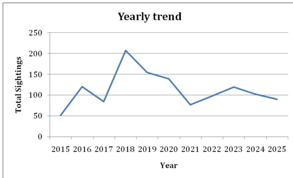
Figure 30: Yearly trend in occurrence of Bar-headed Goose
